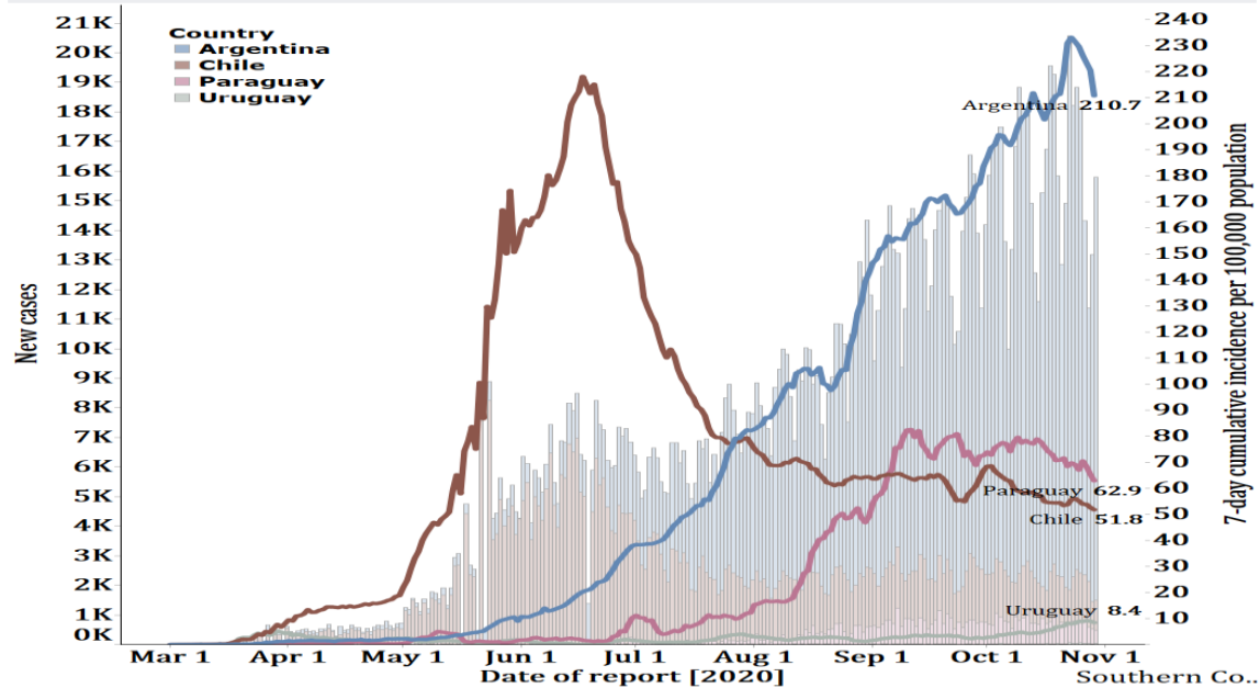
COVID-19 cases and 7-day cumulative incidence per 100,000 pop in Southern Cone, 1 March to 29 October, 2020
