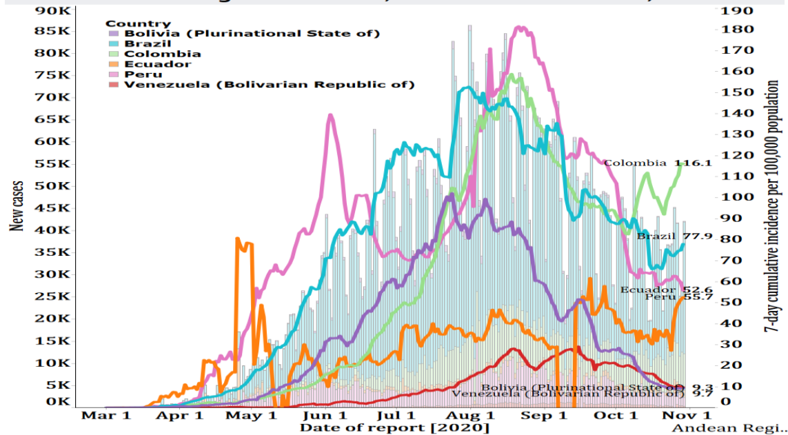
COVID-19 cases and 7-day cumulative incidence per 100,000 pop in Andean Region and Brazil, 1 March to 29 October, 2020
